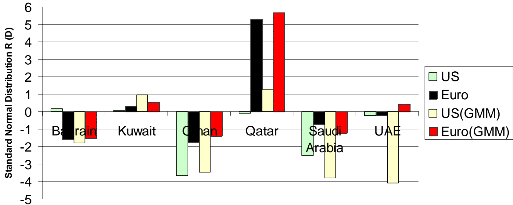
Figure 13: Test Statistic for Sample Generalized Variance
